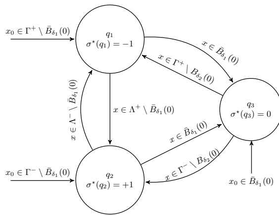
Fig. 6: Finite state machine representing the proposed controller.
