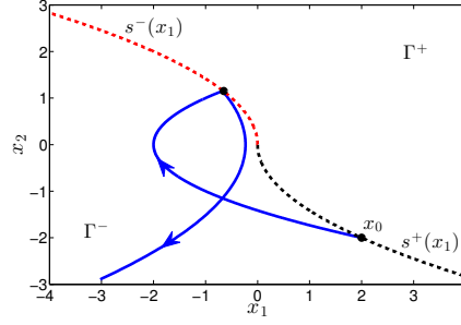
Fig. 4: Loss of stability with d(t) \equiv -\bar{d} .
