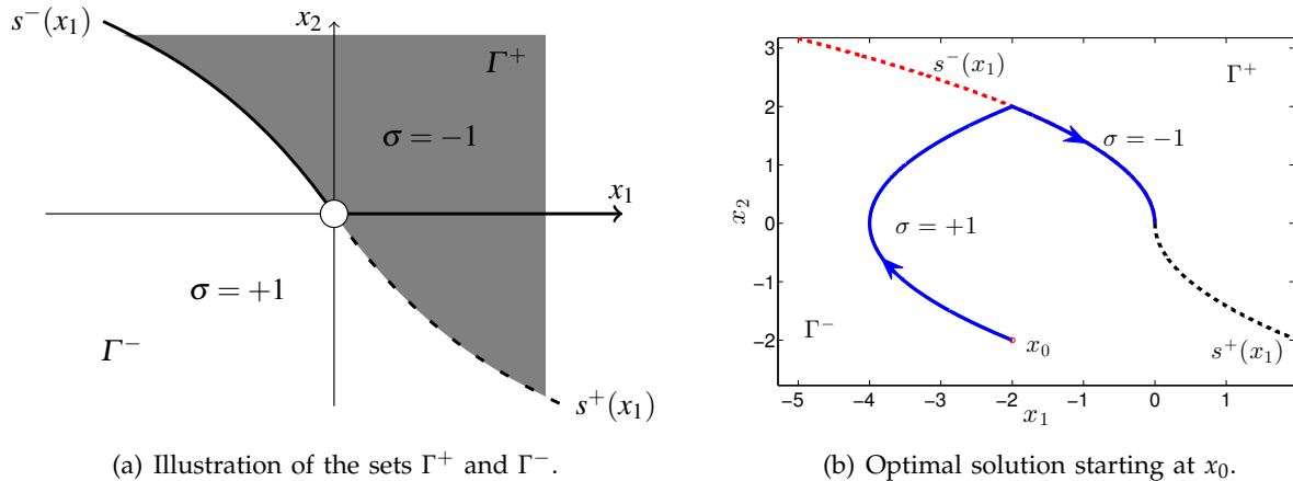
Fig. 2: Time optimal controller for double integrators.
