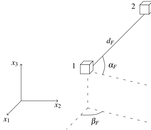
Fig. 1: Illustration of the formation configuration parameters (d_F(t), \alpha_F(t), \beta_F(t)) .
