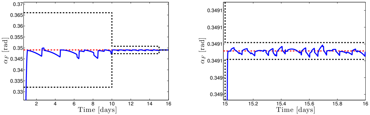
(a) After short transients, \alpha_F(t) is kept, during each phase, (b) After a short transient, \alpha_F(t) is kept in the target bound inside the desired bounds.
