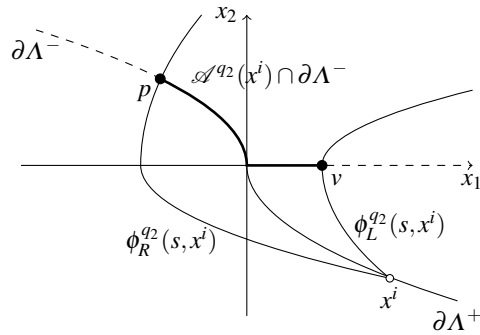
Fig. 9: Attainable switching set from x^i .
