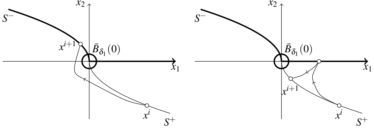
(a) 1-Switch. The state trajectory starts from x^i \in S^+ and hits set \Lambda^- on S^- . (b) 2-Switch. The state trajectory starts from x^i \in S^+ , hits \Lambda^- on the positive x_1 axis and returns to set \Lambda^+ on S^+ .
