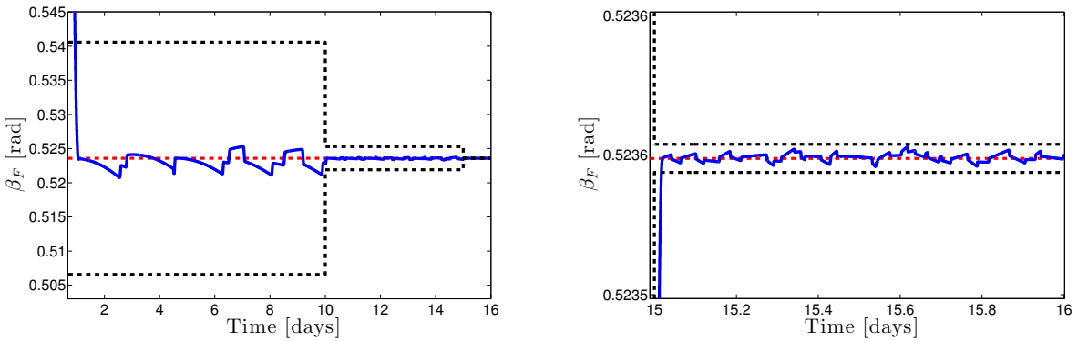
(a) After short transients, \beta_F(t) is kept, during each phase, (b) After a short transient, \beta_F(t) is kept in the target bound inside the desired bounds.
