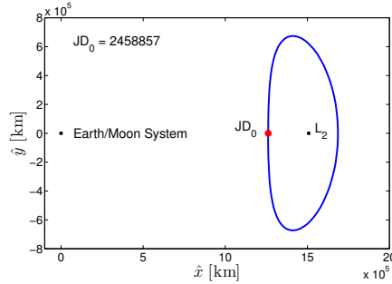
Fig. 11: Nominal Halo orbit in the Sun-Earth/Moon system, as seen in the classical Sun-Earth rotating frame.
