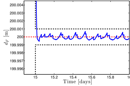
Fig. 15: After a short transient, d_F(t) is kept in the target bound of phase 3.
