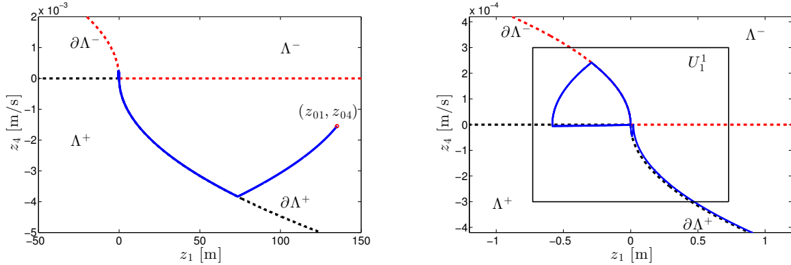
(a) (z_1, z_4) subsystem. The state trajectory approaches a neighborhood of the origin. (b) Formation keeping for phase 1. The state is successfully kept inside the target set.
