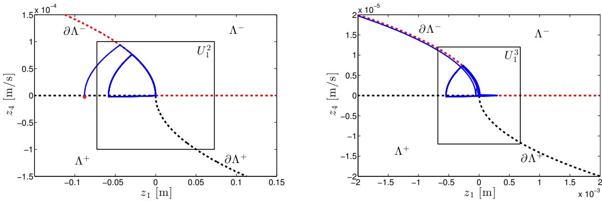
(a) Formation keeping for phase 2. The state is successfully kept inside the target set. (b) Formation keeping for phase 3. The state is successfully kept inside the target set.
