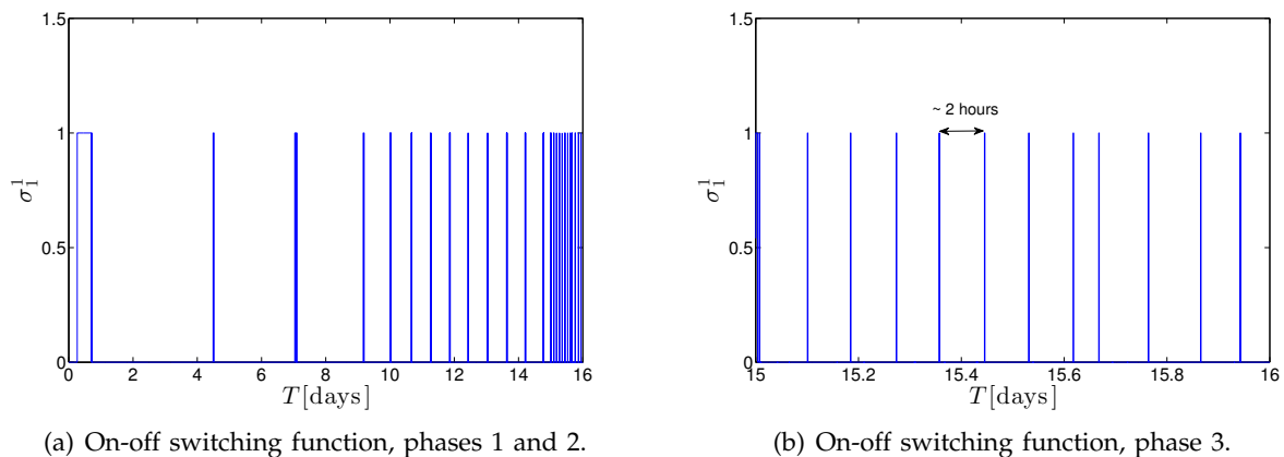
Fig. 19: Switching function for thruster 1.
