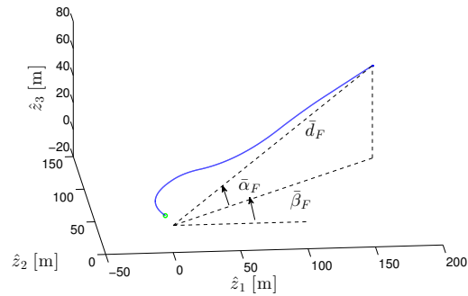
Fig. 18: Trajectory of the follower spacecraft seen by the leader.
