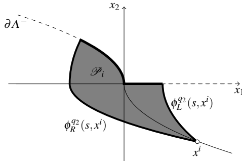
Fig. 10: Set \mathcal{P}_i .
