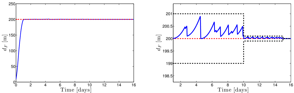
(a) The distance between the spacecraft approaches a neighborhood of \bar{d}_F . (b) After short transients, d_F(t) is kept, during each phase, inside the desired bounds.
