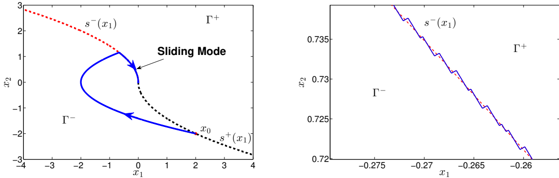
(a) A state trajectory of system (7) when d(t) \equiv -\bar{d} and \sigma is given by (9).
