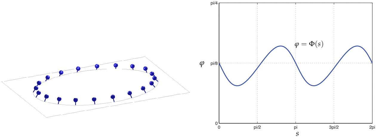
Fig. 2. VHC for the ellipse in Example 3.5.
