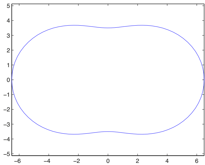
Fig. 6. The non-convex curve considered in example 6.2.
